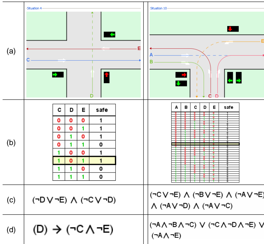
Figure 3.6: Example situations in LogicTraffic
